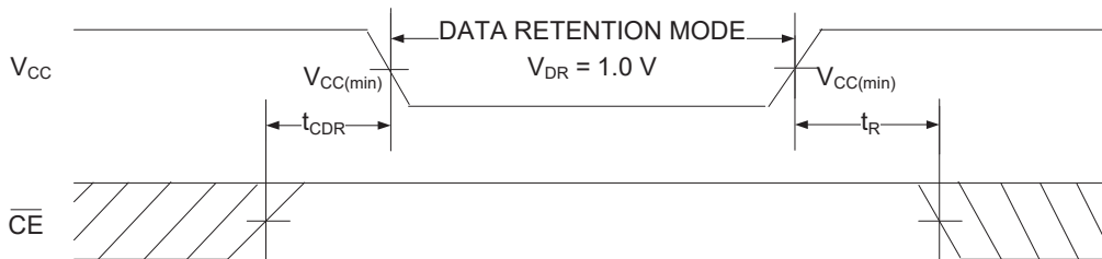
Figure 4. Data Retention Waveform [8]
