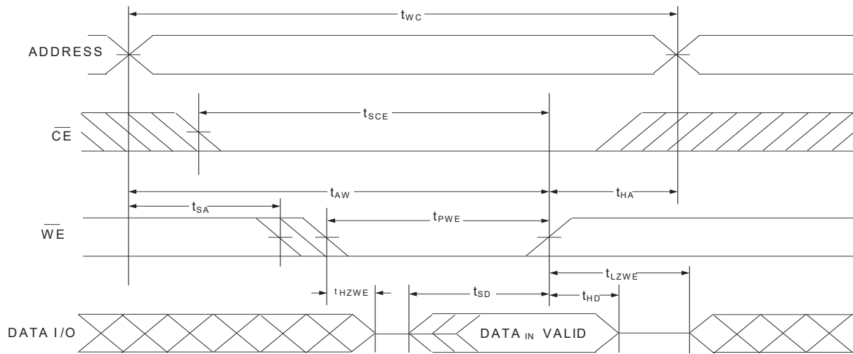
Figure 8. Write Cycle No. 2 ( \overline{WE} Controlled, \overline{OE} LOW) [17, 18, 19]
