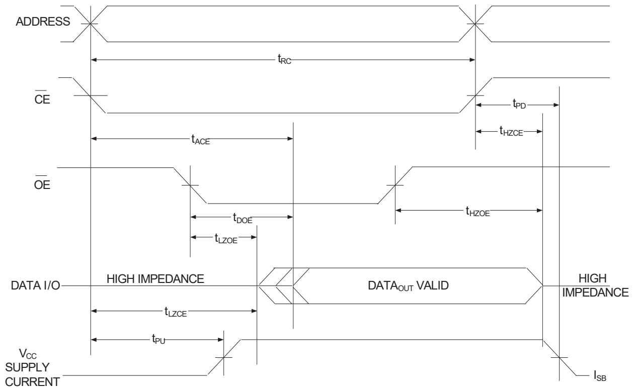
Figure 6. Read Cycle No. 2 ( \overline{OE} Controlled) [15, 16]
