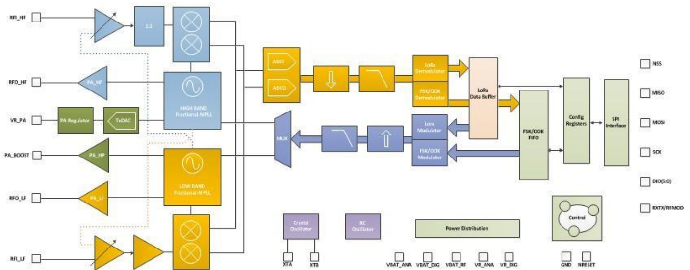
Figure 3. RFM95W/96W/98W Block Schematic Diagram
