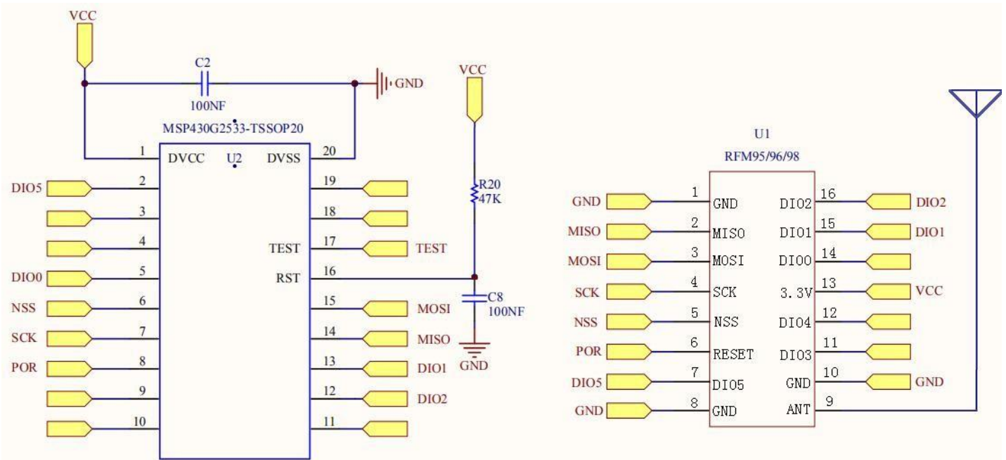
Figure 56:Reference Schematic
